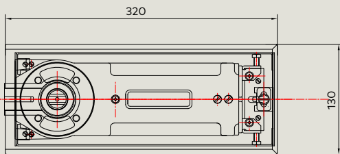
Cement box with dimensions
